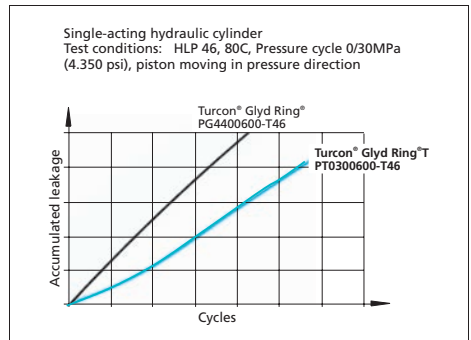
Figure 14 Dynamic leakage Turcon® Glyd Ring® T/ Turcon® Glyd Ring® as single-acting piston seal
