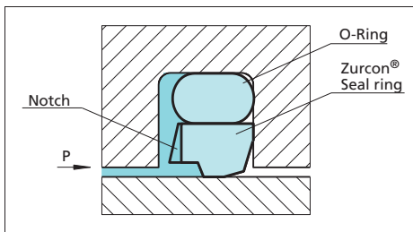
Figure 26 Zurcon® Rimseal
