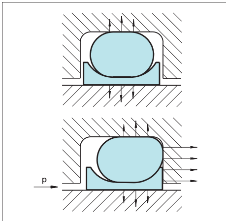
Figure 47 Turcon® Double Delta® with and without pressure
