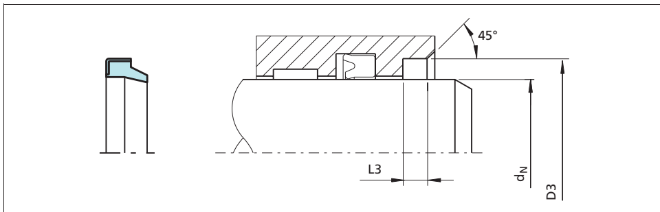
Figure 21 Installation drawing
