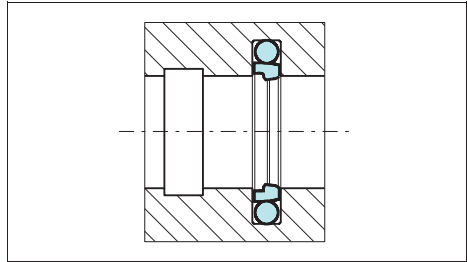
Figure 8 Installation in a closed groove
