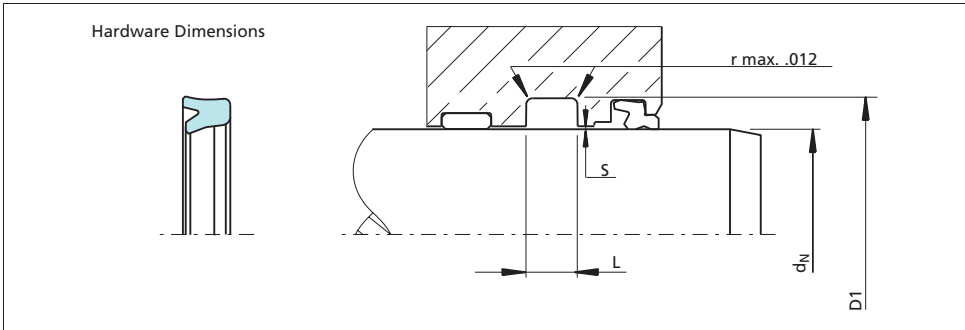
Figure 24 Installation drawing Gap measure "S" see in Table XIII
