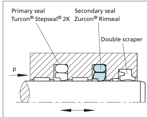
Figure 27 Zurcon® Rimseal in tandem configuration
