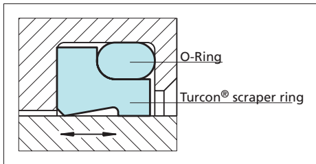
Figure 9 Turcon® Excluder® 2
