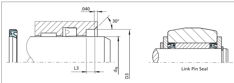
Figure 19 Installation drawing
