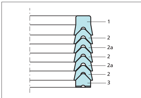
Figure 51 Veepac design
