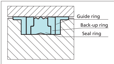
Figure 53 D-A-S Compact Seal, Type A
