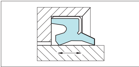
Figure 5 Scraper WKE
