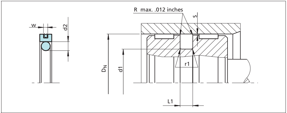
Figure 43 Installation drawing
