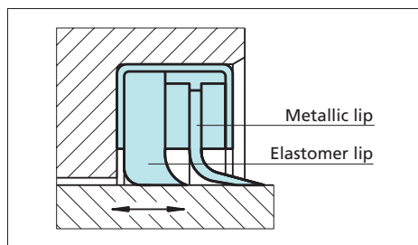
Figure 22 Metal Scraper
