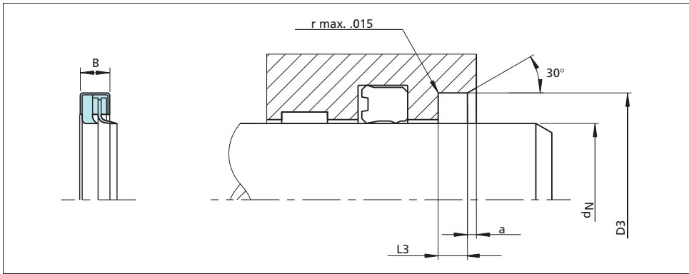
Figure 23 Installation drawing
