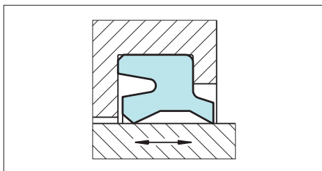
Figure 1 Scraper DA 22
