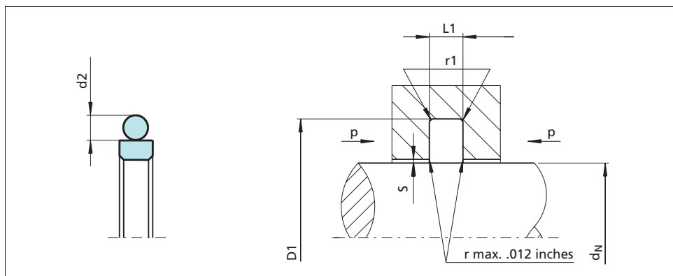
Figure 38 Installation drawing
