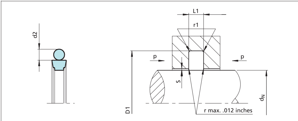
Figure 35 Installation drawing
