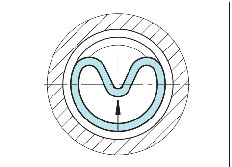
Figure 7 Inserting the seal ring into the closed groove
