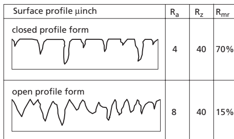
Figure 2 Profile forms of surfaces
