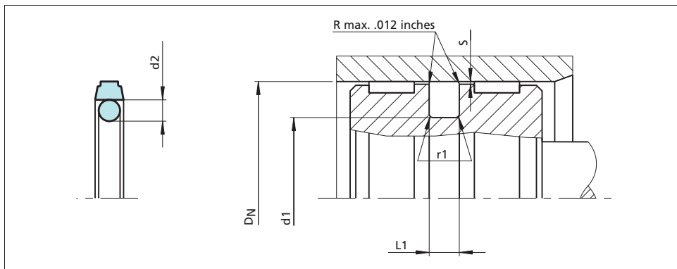
Figure 15 Installation drawing
