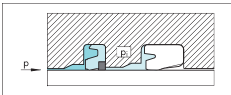
Figure 29 Tandem configuration
