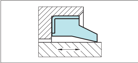
Figure 20 Scraper WSA
