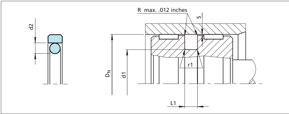
Figure 25 Installation drawing
