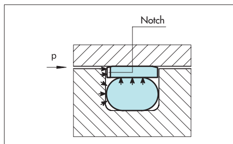
Figure 27 Turcon® Glyd Ring® C with notches on both sides
