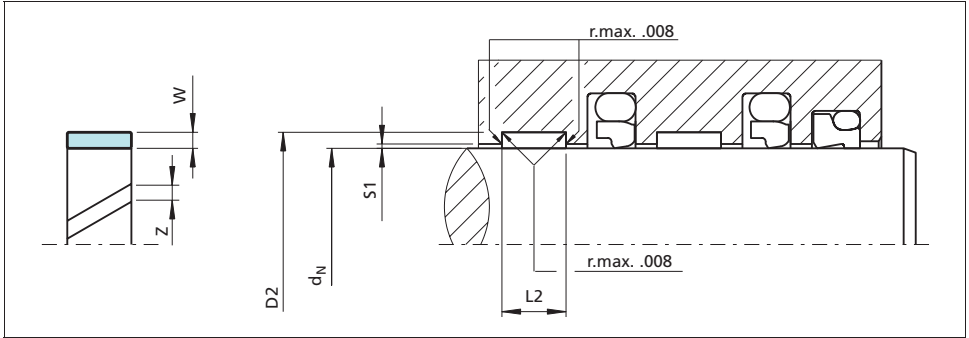
Figure 4 Installation drawing
