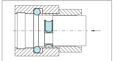
Figure 12 Insertion with an inserter tube
