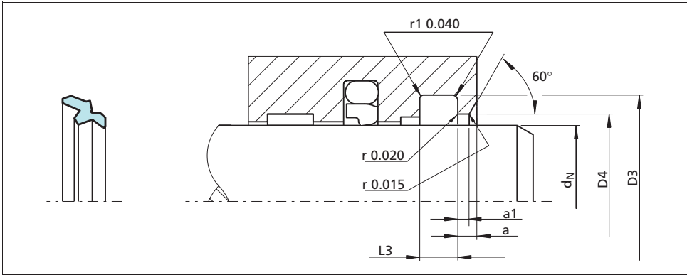
Figure 4 Installation drawing
