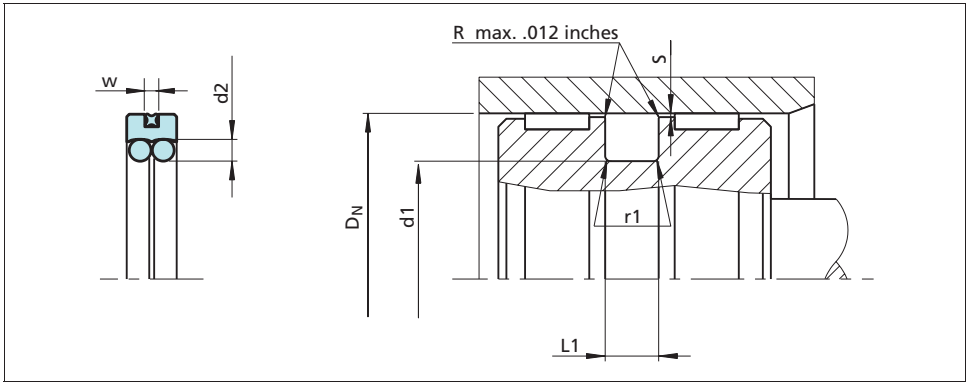
Figure 45 Installation drawing
