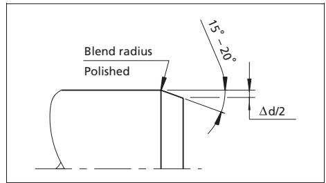
Figure 2 Lead-in chamfers
