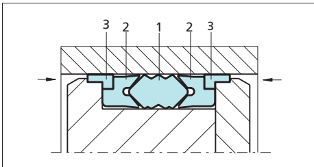
Figure 56 Selemaster design
