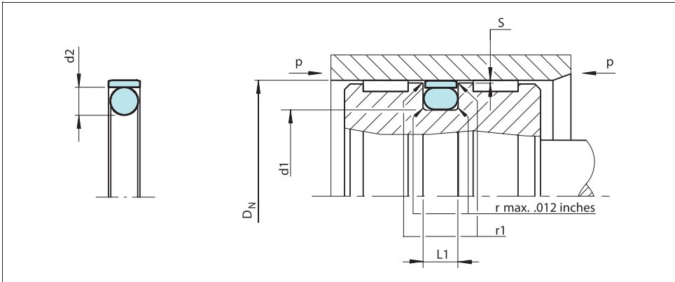
Figure 29 Installation drawing
